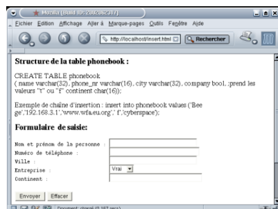
Figure 43.2. Formulaire insert.html
