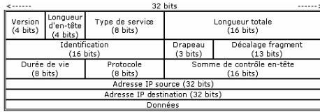
Figure 1.2. datagramme IP
