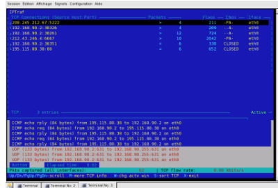
Figure 64.1. iptraf
