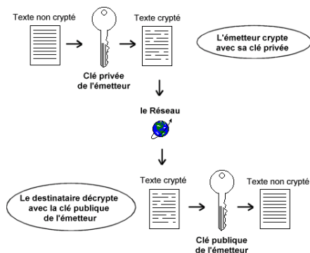
Figure 23.3. Authentification
