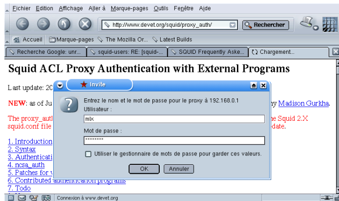
Figure 41.3. Authentification SQUID
