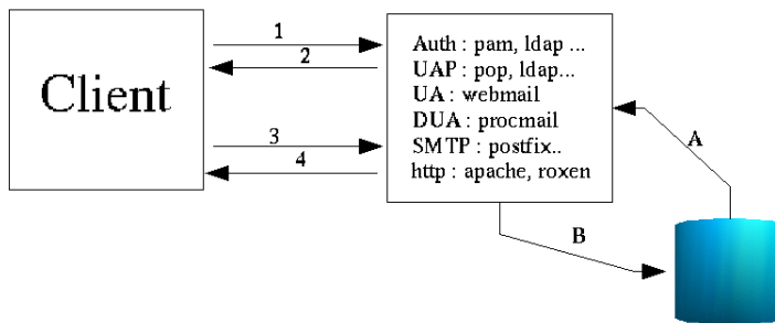
Figure 39.1. Architecture globale d'un service Web-mail
