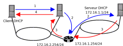
Figure 29.1. Dialogue client DHCP, agent de relai DHCP et serveur DHCP
