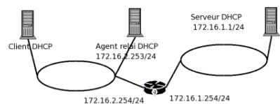
Figure 29.2. Maquette agent relais DHCP
