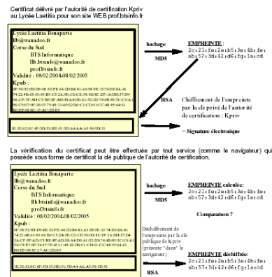
Figure 23.5. Certificat
